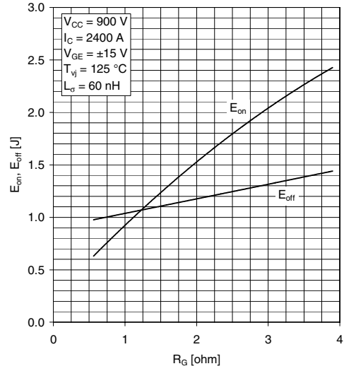
Fig. 8 Typical switching energies per pulse vs gate resistor
